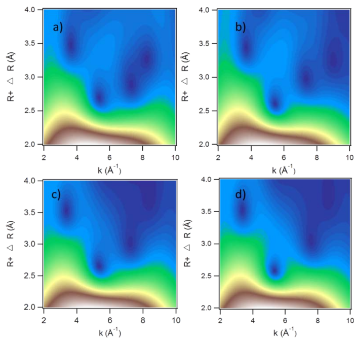
Fig S2. Wavelet transforms of spectra and models Cd(II) bound to ferrihydrite with phosphate added. The k -range used was 2.6-9.5 \text{\AA}^{-1} for all samples. a) Spectrum H3; 30 \mu\text{mol L}^{-1} Cd, 3 \text{mmol L}^{-1} Fe, 600 \mu\text{M} P, b) Spectrum H8; 30 \mu\text{mol L}^{-1} Cd, 0.3 \text{mmol L}^{-1} Fe, 60 \mu\text{mol L}^{-1} P, c) Model H3, d) Model H8.
