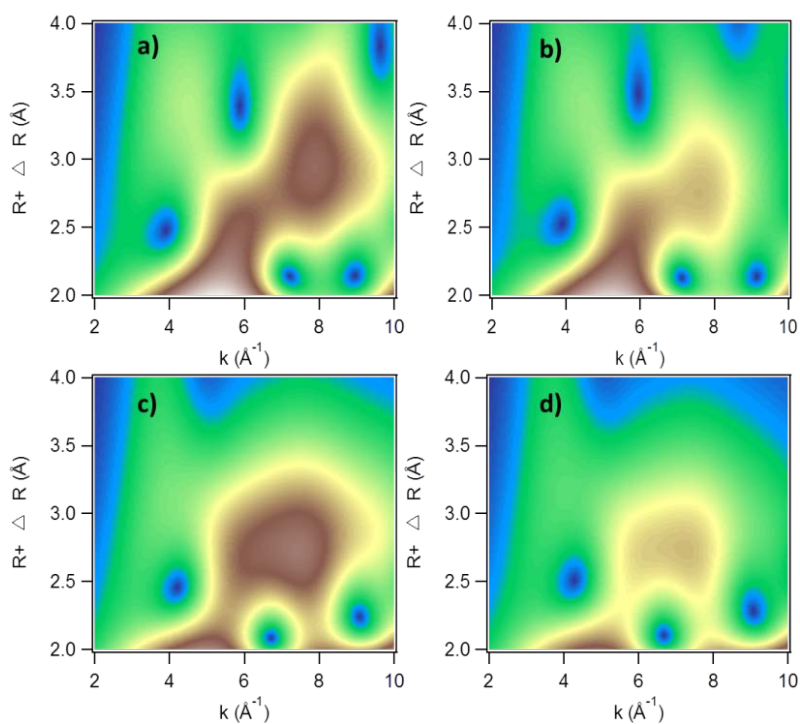
Fig S6. Wavelet transforms of EXAFS spectra and models for arsenic adsorbed to ferrihydrite. The k -range used was 3.6-12.5 \text{\AA}^{-1} for all samples. a) Spectrum I11; 60 \mu\text{mol L}^{-1} As, 0.3 \text{mmol L}^{-1} Fe, b) Spectrum H12b; 60 \mu\text{mol L}^{-1} As, 0.3 \text{mmol L}^{-1} Fe, 30 \mu\text{mol L}^{-1} Cd, c) Model I11, d) Model H12b.
