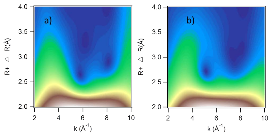
Fig S4. Wavelet transform of EXAFS spectra and model for cadmium(II) solution a) Spectrum 15 \text{mmol L}^{-1} \text{Cd}(\text{NO}_3)_2(\text{aq}) , b) Model 15 \text{mmol L}^{-1} \text{Cd}(\text{NO}_3)_2(\text{aq}) , The k -range used was 3-10 \text{\AA}^{-1} .
