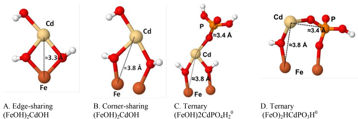
Fig 5. Structures of cadmium(II) surface complexes consistent with both EXAFS interpretations and SCM results. Bright red atoms are oxygen and white atoms are hydrogen. Iron, cadmium(II) and phosphorus atoms are marked. The Cd···Fe and Cd···P distances from the EXAFS analysis are shown. Structures of the ternary cadmium(II)-arsenate complexes are similar except that the Cd···As distance is 3.5 Å.
