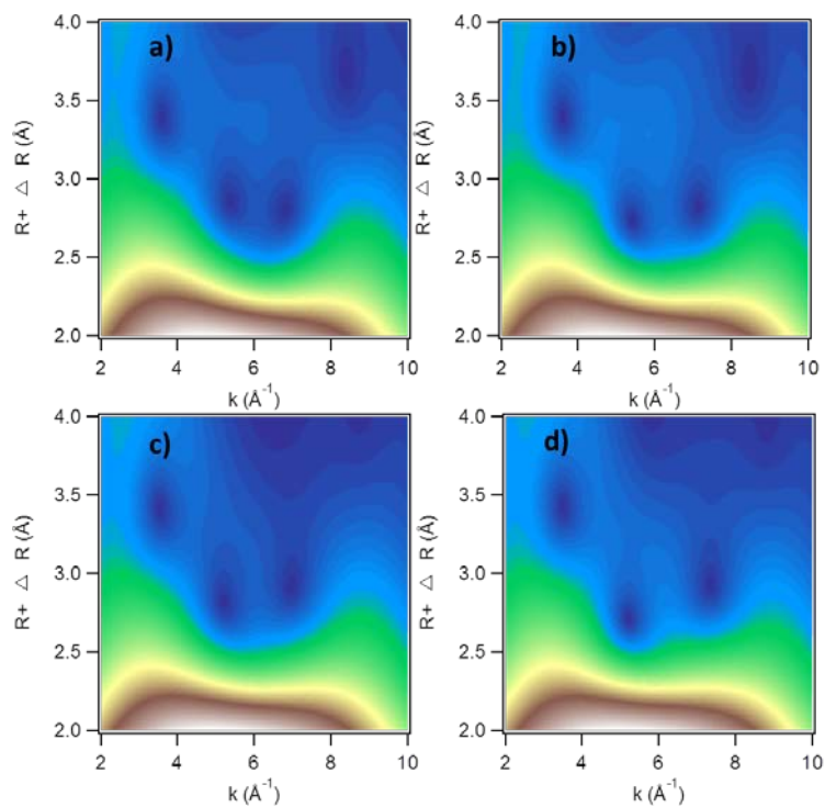
Fig S3. Wavelet transforms of spectra and models Cd(II) bound to ferrihydrite with arsenate added. The k -range used was 2.6-9.5 \text{\AA}^{-1} for all samples. a) Spectrum H10; 30 \mu\text{mol L}^{-1} Cd, 3 \text{mmol L}^{-1} Fe, 600 \mu\text{mol L}^{-1} As, b) Spectrum H12; 30 \mu\text{mol L}^{-1} Cd, 0.3 \text{mmol L}^{-1} Fe, 60 \mu\text{mol L}^{-1} As, c) Model H10, d) Model H12.
