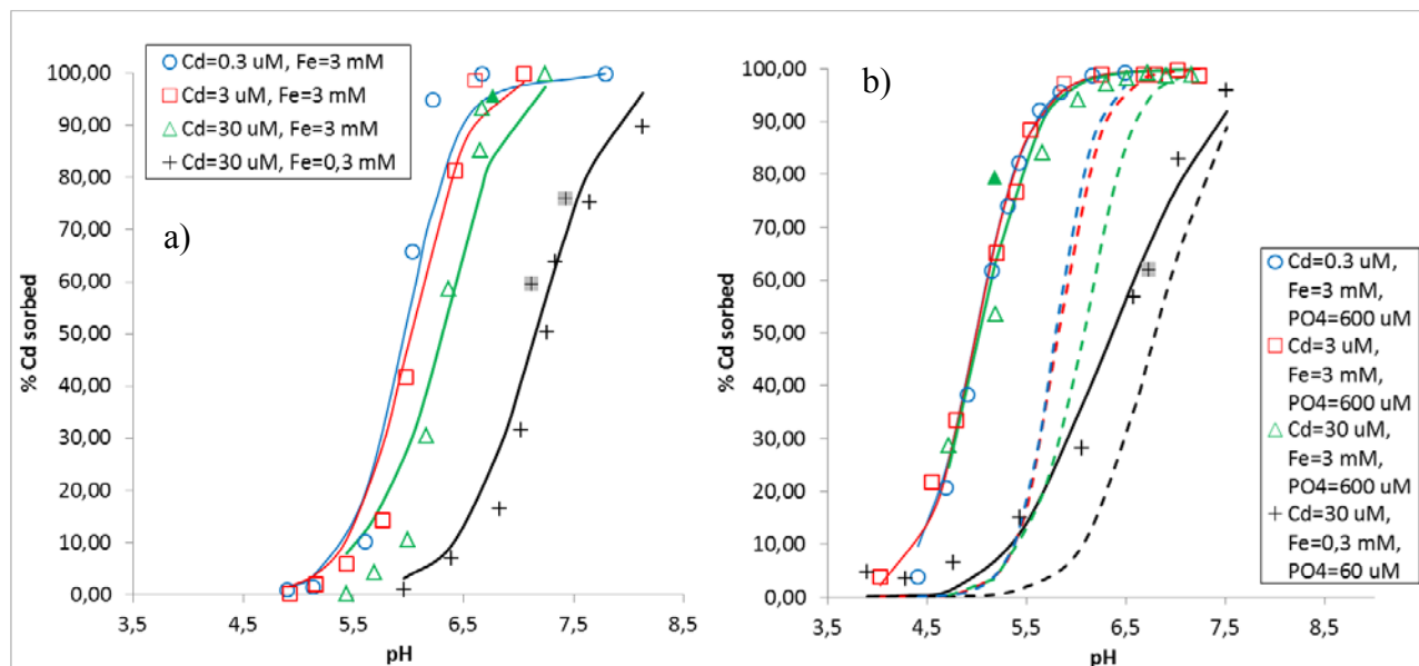
Fig 1. Cadmium(II) sorption to ferrihydrite at Cd/Fe ratios 0.0001, 0.001, 0.01 and 0.1. Results from batch experiments (symbols) and SCM (lines) with the optimized parameters from Table 1. Filled symbols are samples for EXAFS measurements. a) Only cadmium(II) and ferrihydrite. b) With phosphate added; model without ternary surface complex (dashed lines) and with ternary complex (solid lines).
