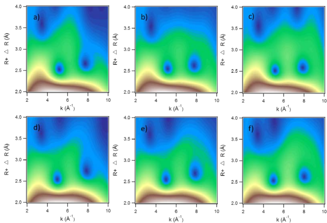
Fig S1. Wavelet transforms of EXAFS spectra and models for cadmium(II) bound to ferrihydrite. The k -range used was 2.6-9.5 \text{\AA}^{-1} . a) Spectrum H2; 30 \mu\text{mol L}^{-1} Cd, 3 \text{mmol L}^{-1} Fe, b) Spectrum H6; 30 \mu\text{mol L}^{-1} Cd, 0.3 \text{mmol L}^{-1} Fe, c) Spectrum H7; 30 \mu\text{mol L}^{-1} Cd, 0.3 \text{mmol L}^{-1} Fe, d) Model H2, e) Model H6, f) Model H7.
