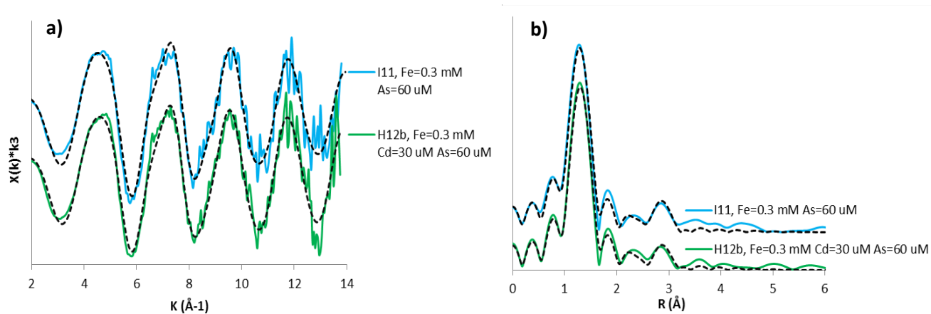
Fig S5. Results from EXAFS-measurements (solid lines) and models (dashed lines) at the As K edge. a) EXAFS spectra, b) Fourier transforms.
