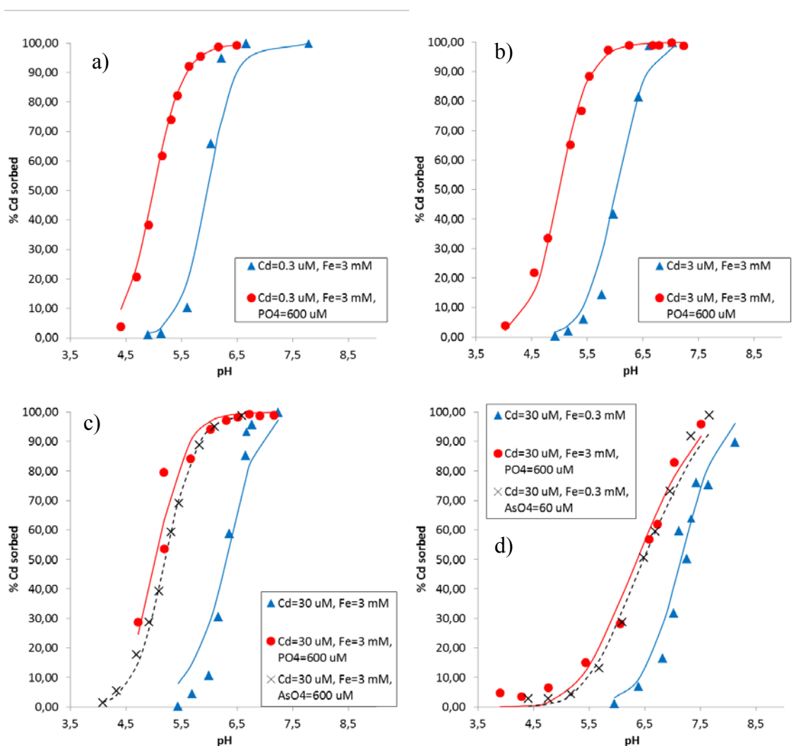
Fig 3. Sorption of cadmium(II) to ferrihydrite (blue symbols), with phosphate added (red symbols) and with arsenate added (black symbols). Lines are SCM results with the optimized parameters from Table 1. a) Cd/Fe ratio 0.0001, b) Cd/Fe ratio 0.001, c) Cd/Fe ratio 0.01 and d) Cd/Fe ratio 0.1.
