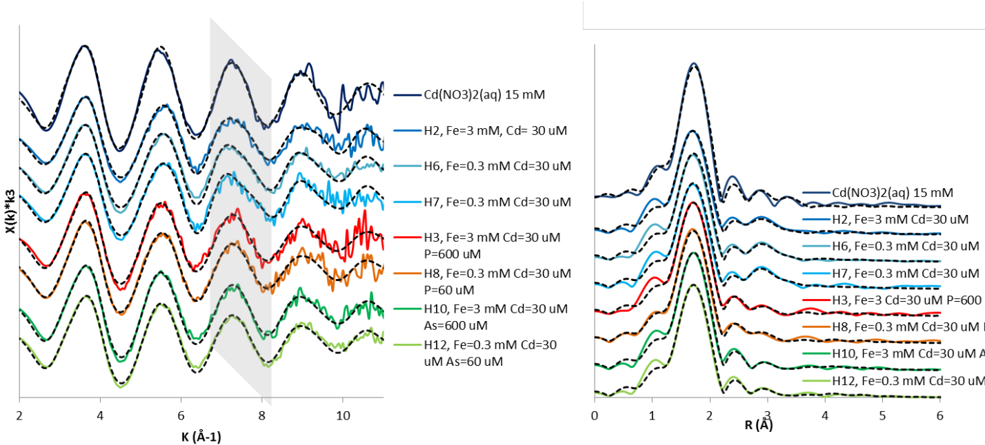
Fig 4. Results from EXAFS measurements of cadmium(II) adsorbed to ferrihydrite and \text{Cd}(\text{NO}_3)_2 solution. a) EXAFS spectra (solid lines) and model fits (dashed lines). b) Fourier transforms of EXAFS spectra (solid lines) and model fits (dashed lines). The shaded area highlights an area where spectra for sample H2, H6 and H7 have a different shape than spectra from H3, H10 and H12.
