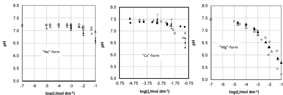
Figure 18. Potentiometric electrolyte titrations of ACF2944. (a) Na + -form with NaCl ( \Delta ), \text{LiNO}_3 ( \circ ), and CsCl ( \diamond ) and end points of mass titration ( \blacktriangle with error bars); (b) Ca 2+ -form with NaCl ( \Delta ), \text{Ca}(\text{NO}_3)_2 ( \blacksquare ), and \text{CaCl}_2 ( \square ) and end points of mass titration ( \blacklozenge with error bars); and (c) Mg 2+ -form with NaCl ( \Delta ), \text{NaNO}_3 ( \blacktriangle ), \text{LiNO}_3 ( \circ ), and CsCl ( \diamond ).
