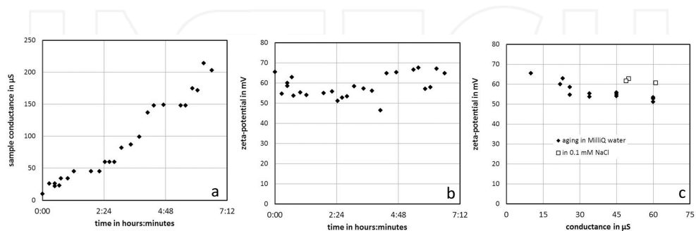
Figure 6. (a) Conductance of a gibbsite suspension in MilliQ water at pH 5.6 as a function of time. (b) Zeta-potential of a gibbsite suspension in MilliQ water at pH 5.6. (c) Zeta-potential of a gibbsite sample in MilliQ water when aged as a function of the conductance in comparison to a sample in 0.1 mM NaCl yielding a conductance in the relevant range.
