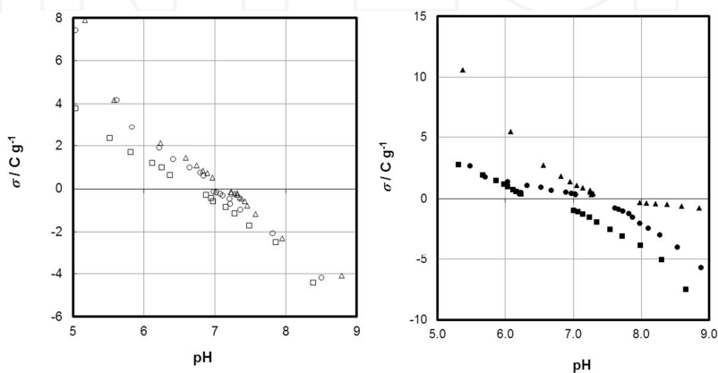
Figure 17. (a) Surface charge density of ACF2944 (Na-form) (calculated from mass titration data shown on Figure 15) at different ionic strength: I_c (mol/dm 3 ): 0.001 (Δ), 0.01 (○), and 0.1 (□); NaCl; t=20^{\circ}\text{C} . (b) Surface charge density of ACF2944 (Ca-form) (calculated from mass titration data shown on Figure 16) at different ionic strength: I_c (mol/dm 3 ): 0.00033 (▲), 0.0033 (●), and 0.033 (■). Ionic strength was controlled by CaCl 2 ; t=20^{\circ}\text{C} .
