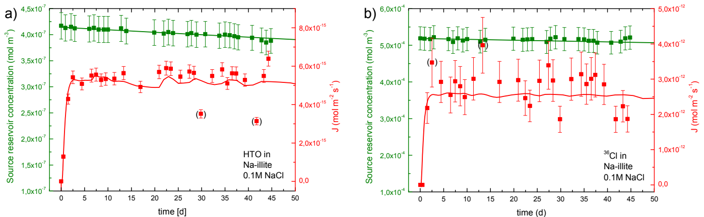
Figure 38 Diffusion of HTO (a) and ^{36}Cl (b) in compacted Na-illite ( \rho_{db} \sim 1700 kg m^{-3} ) at pH 5.5 and 0.1 M NaCl as mass flux in the low concentration reservoir ( J ) and evolution of the source reservoir concentration.
