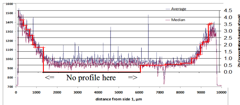
Figure 73 Comparison of the Zn profile obtained by \mu Libs (blue and purple curves) and by abrasive-peeling (red curve).
