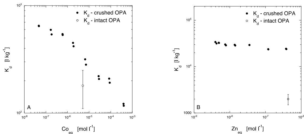
Figure 62 Comparison between sorption of \text{Co}(\text{II}) (left) and \text{Zn}(\text{II}) (right) measured on crushed Opalinus Clay (filled symbols, isotherm) and sorption derived from the diffusion experiment on intact Opalinus Clay (open symbols).
