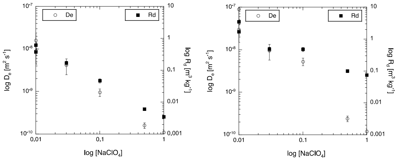
Figure 52 Dependence of D_e and R_d for ^{85}\text{Sr}^{2+} on the \text{NaClO}_4 concentration in the contacting solution for the experiments at pH 5 (left-hand plot) and the experiments at pH 9 (right-hand plot).
