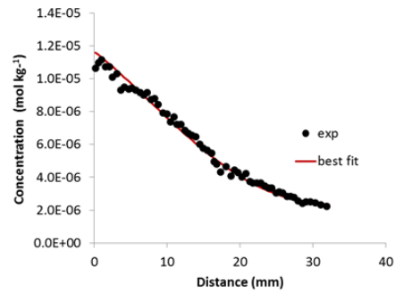
Concentration in the clay profile ( \text{mol kg}^{-1} )
