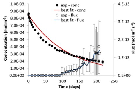
Concentration in the source reservoir ( \text{mol m}^{-3} ) and flux in the target reservoir ( \text{mol m}^{-2} \text{s}^{-1} )
