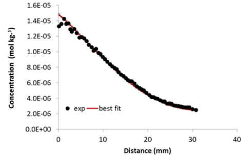
Concentration in the clay profile ( \text{mol kg}^{-1} )
