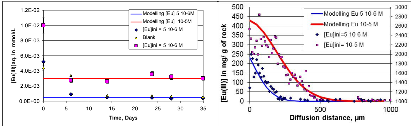
Figure 83 Comparison of the experimental Eu data from the cells with [Eu(III)]_{ini} = 5 \times 10^{-6} M (blue curves) and [Eu(III)]_{ini} = 10^{-5} M (red curves) with modeling in the reservoir (left) and the rock profile (right).
