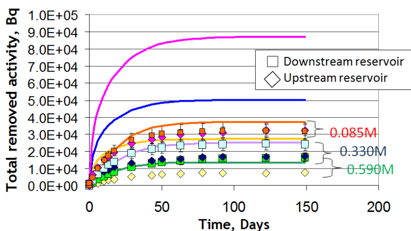
Figure 70 Evolution of the ^{85}\text{Sr} activity in the up- and downstream reservoirs of the three cells during the out-diffusion stage. Curves were modelled by means of analytical approach using the diffusive parameters determined from through-diffusion experiments and given in Table 38.
