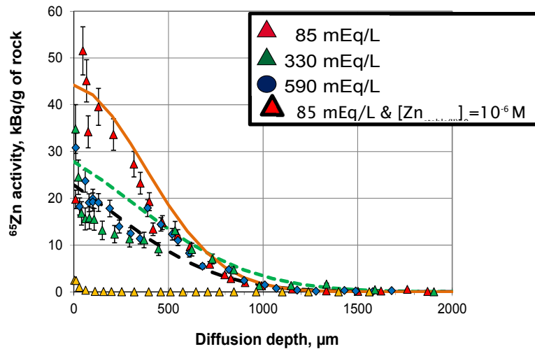
Figure 77 ^{65}\text{Zn} rock profile acquired on the four cells and the associated modelled curves.
