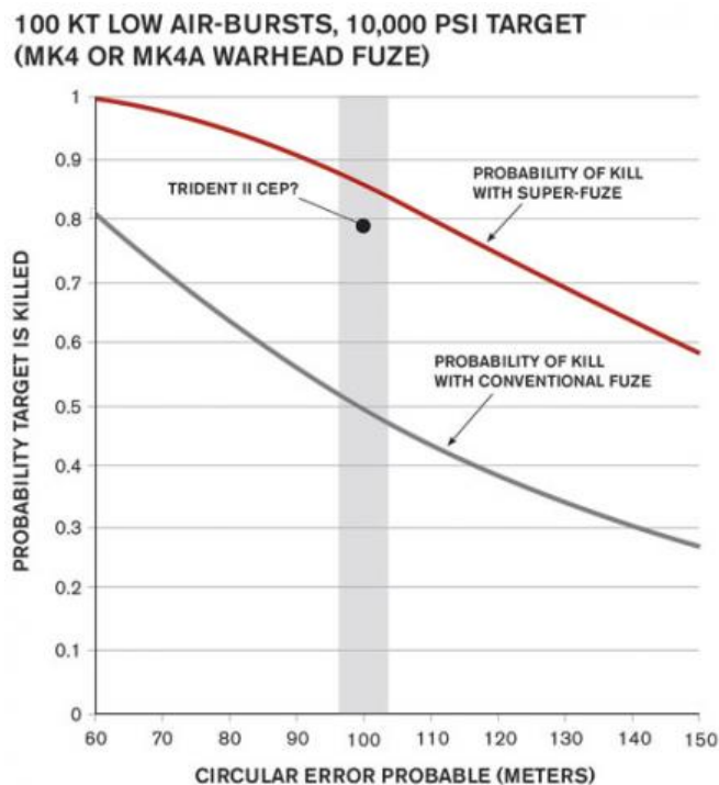
FIGURE 4. The probability of destroying a fully hardened Russian target with the super-fuzed W76-1/Mk4A warhead atop an American submarine-launched ballistic missile is about 86 percent—far higher than would be the case with the previous fuzing for the warhead.
