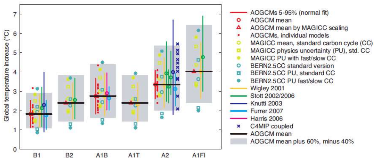
Figure 1. Projections and uncertainties for global mean temperature change in 2090-2099 relative to the 1980-1999 average, under several emission scenarios and from numerous studies. The 5-95% ranges from probabilistic studies are indicated by solid vertical lines. The IPCC “likely” ranges are indicated by the wide grey bars. (Reprinted from Climate Change 2007: The Physical Science Basis. Working Group I Contribution to the Fourth Assessment Report of the Intergovernmental Panel on Climate Change , Figure 10.29. Cambridge University Press.)
