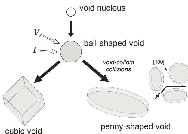
Figure 7.11: The scheme of the voids development stages.
