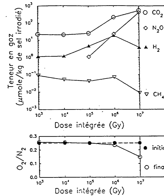
Figure 11 Gas production vs integrated dose : Grain size between 1 mm and 2 mm ( 10^4 Gy/h in air @ 50^\circ\text{C} )
