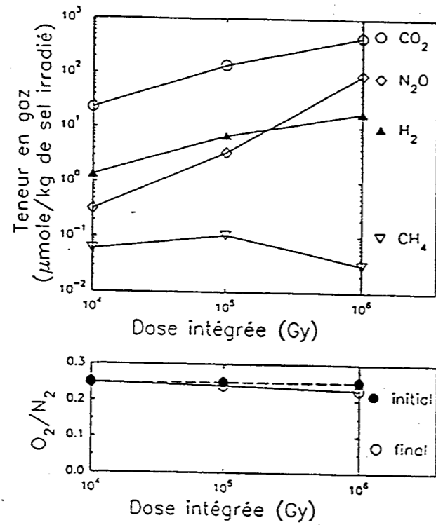
Figure 9 Gas production vs integrated dose ( 10^4 Gy/h in air @ 200^\circ\text{C} )
