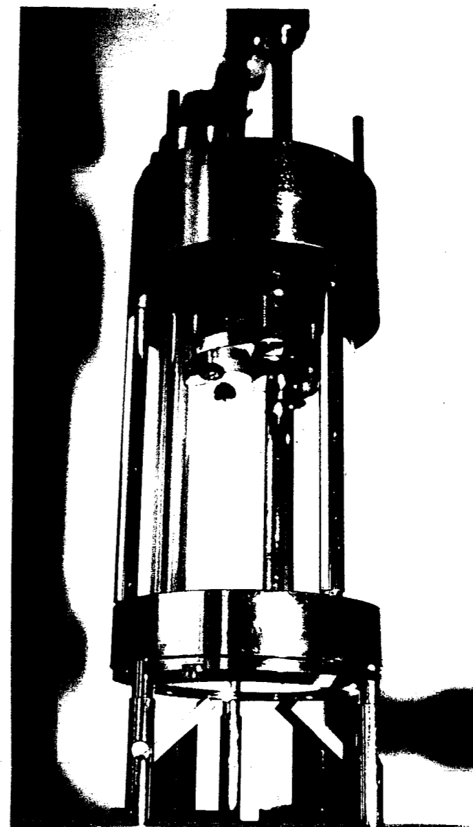
Figure 3 : Cell developed for FTIR spectroscopy
