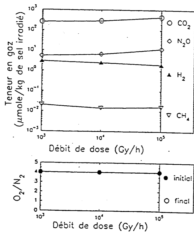
Figure 18 Gas production vs dose rate : Initial filling gas 20% N 2 + 80% O 2 (10 6 Gy @ 50°C)
