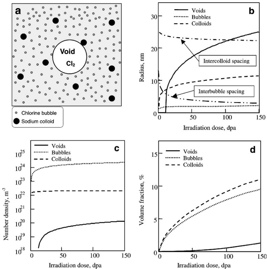
Fig. 2. Evolution of bubbles, colloids and voids with increasing irradiation dose (in displacements per anion, dpa) calculated for the laboratory irradiation conditions (100 °C, 3 \times 10^{-5} dpa/s) and a constant dislocation density 10^{14} \text{ m}^{-2} [14]. (a) Graphic illustration; (b) Intersection between the colloid radius and interbubble spacing curves indicates a beginning of the explosive back reaction due to collisions between the bubbles and colloids resulting in the formation of voids, which grow to sizes exceeding the intercolloid spacing and thus provide for the following and larger step of the explosive back reaction; (c) and (d) show the corresponding number densities and volume fractions of radiolytic products.
