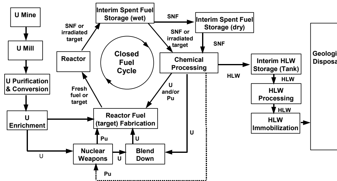
FIGURE 1.1 Material-flow diagram of a closed nuclear fuel cycle. A plutonium-production process diagram has nearly identical components except that the reactor irradiates uranium targets, which are processed to recover Pu (see the dotted line from chemical processing to nuclear weapons).
