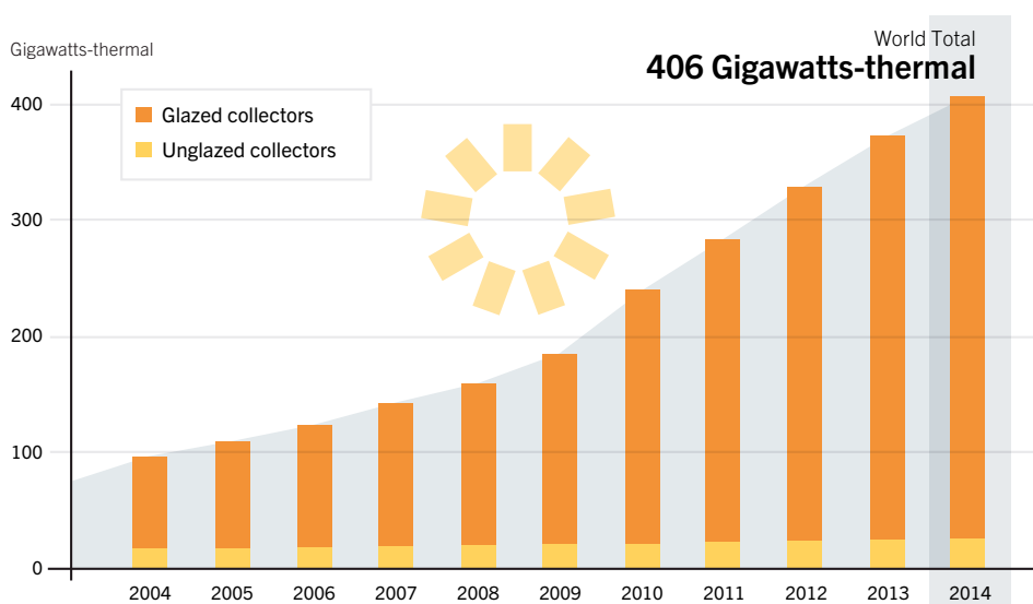
Figure 21. Solar Water Heating Collectors Global Capacity, 2004–2014
