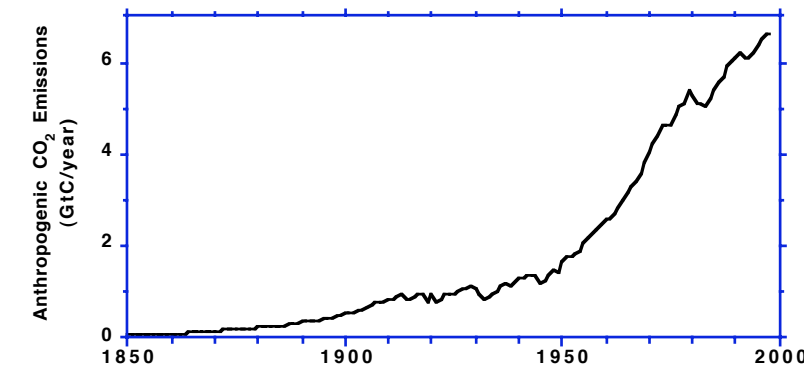
Figure 1. Global CO 2 emissions resulting from human activity (billion tons of carbon per year)
