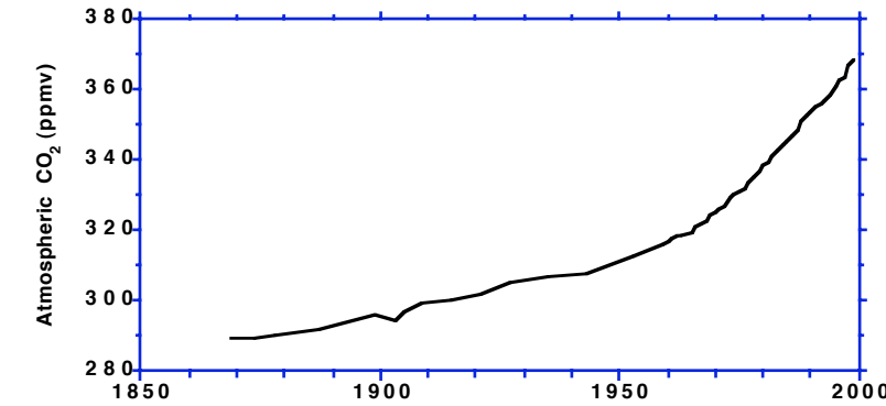
Figure 2. Atmospheric CO 2 concentrations, parts per million.
